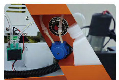
6. Ink pump/White ink circulation pump/White ink stirring
