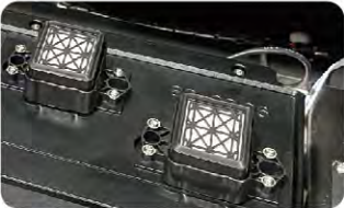
Elevation Capping Station
